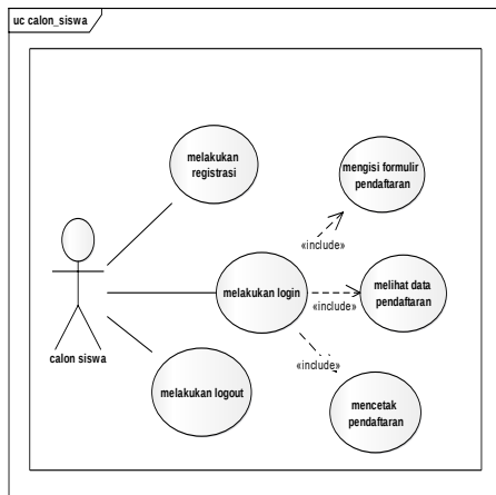
Gambar 1. Use Case Diagram Halaman PPDB
