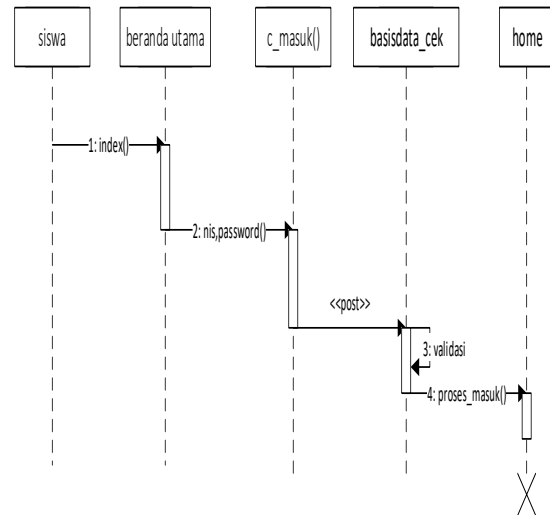
Gambar 12. Sequence Diagram login user
