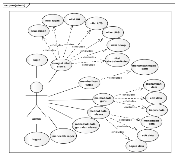
Gambar 4. Use Case Diagram Halaman Guru(admin)
