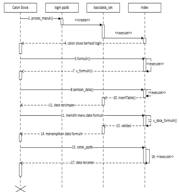
Gambar 13. Sequence Diagram registrasi
