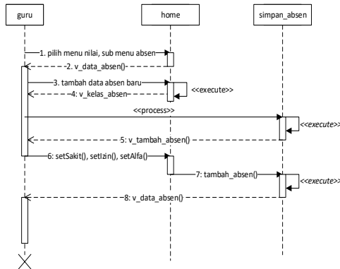
Gambar 14. Sequence Diagram Nilai
