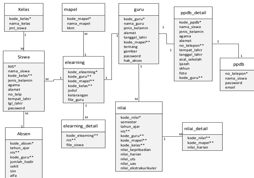
Gambar 10. Logical Record Structure (LRS)
