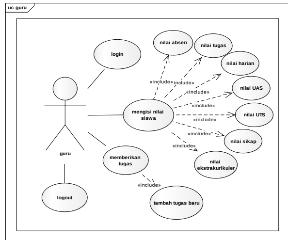
Gambar 3. Use Case Diagram Halaman Guru Table 3. Deskripsi Use Case Diagram Halaman Guru
