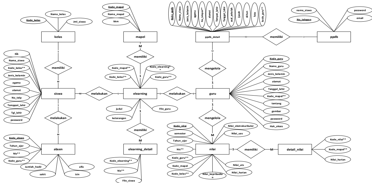
Gambar 9. Entity Relational Diagram
