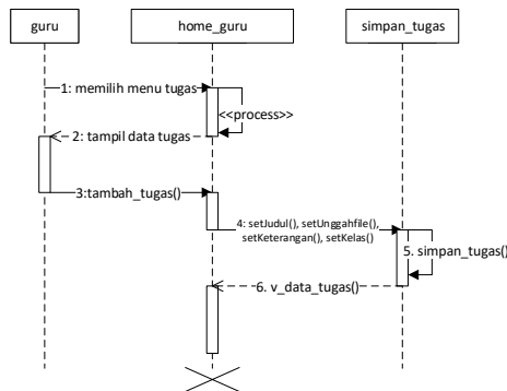
Gambar 15. Sequence Diagram Tugas
